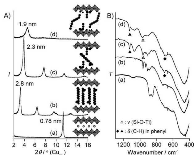
Figure 1. A) X-ray diffraction patterns and B) infrared spectra of KTLO (a), C 12 TMA-TLO (b), PTMS-TLO (c), and PTMS-C 18 TMS-TLO (d). I = intensity, T = transmittance. Inset: Schematic drawings of the corresponding interlayer structures.
